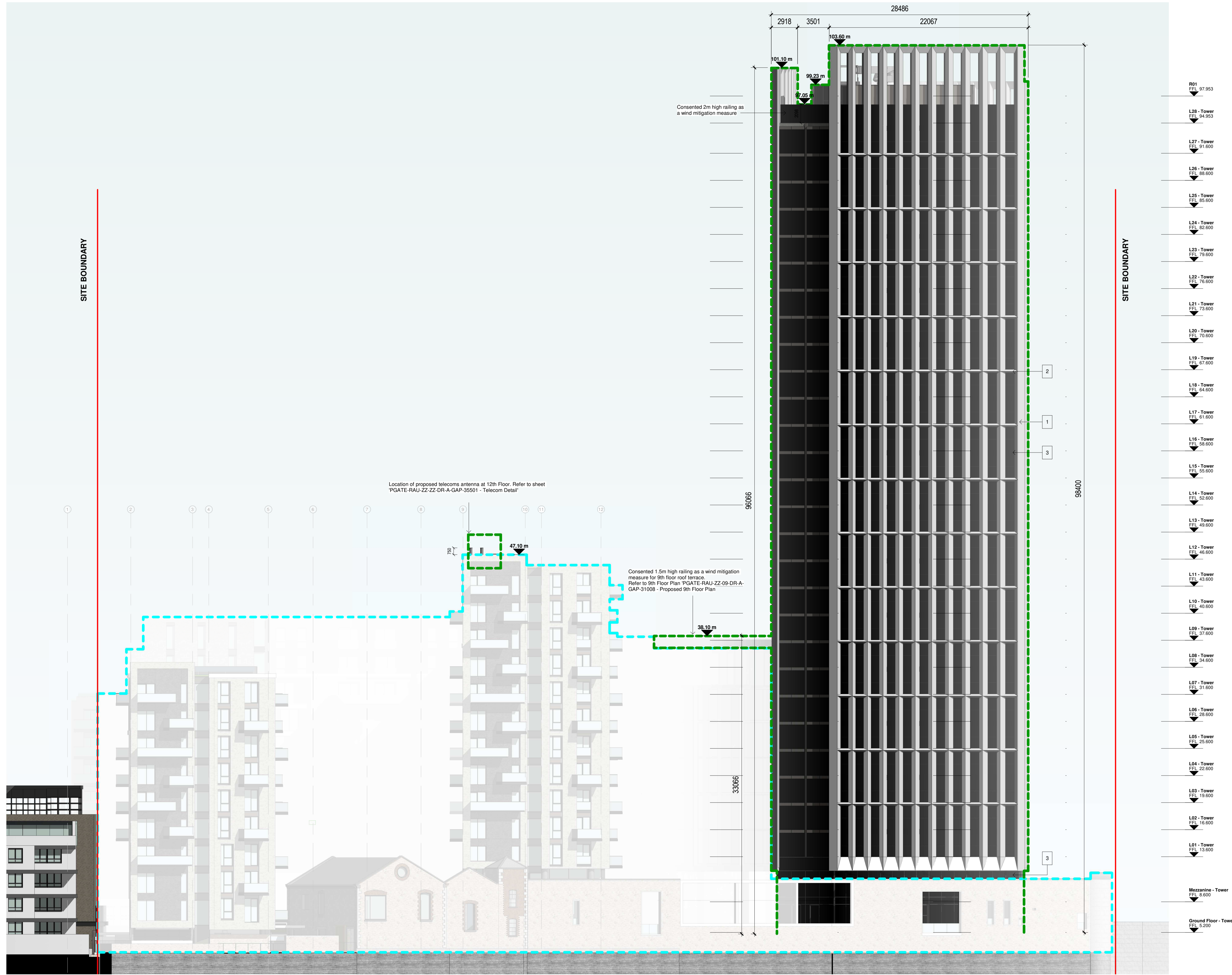
Proposed South Elevation 1 : 200
